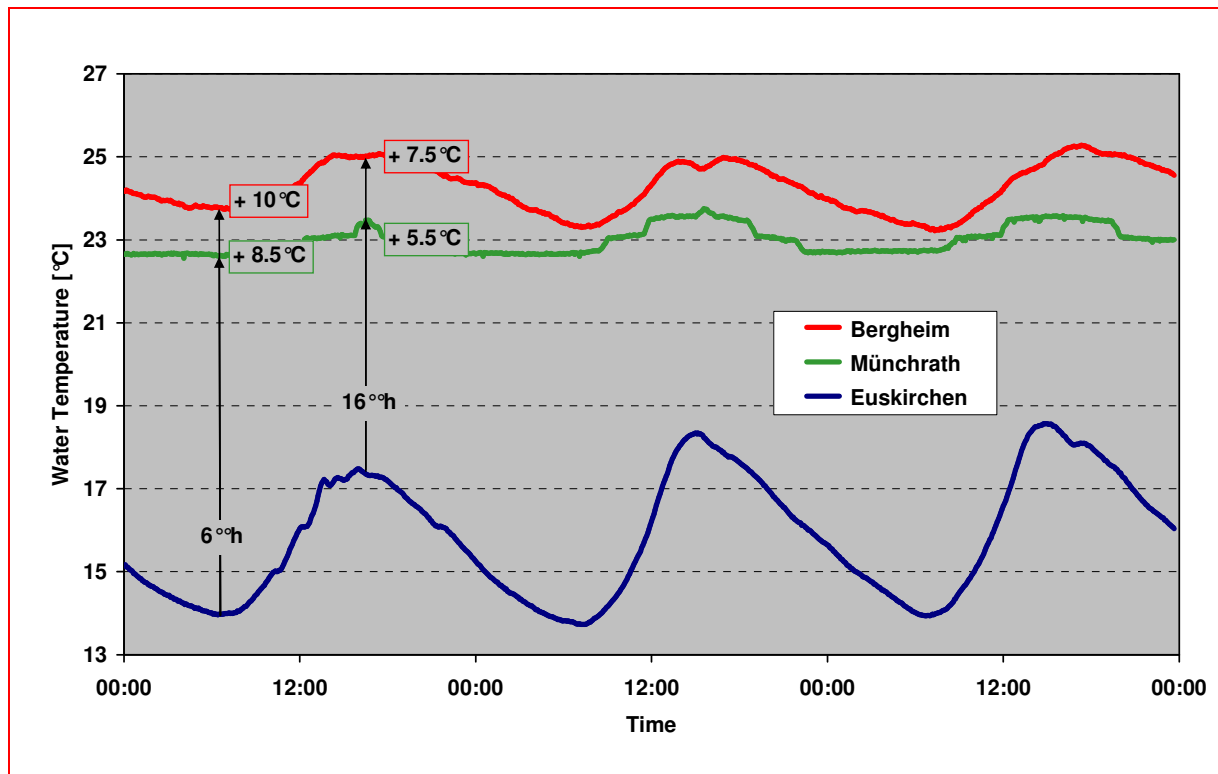
Figure 14: Water Temperature – Diurnal Fluctuations in August at the Upper (Euskirchen), Middle (Bergheim) and Lower (Münchrath) Reaches, Year 2003.
