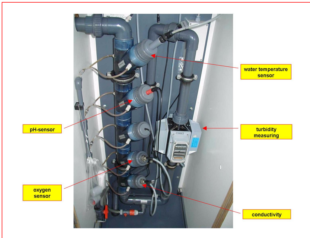
Figure 11: Instrument Cabinet.
