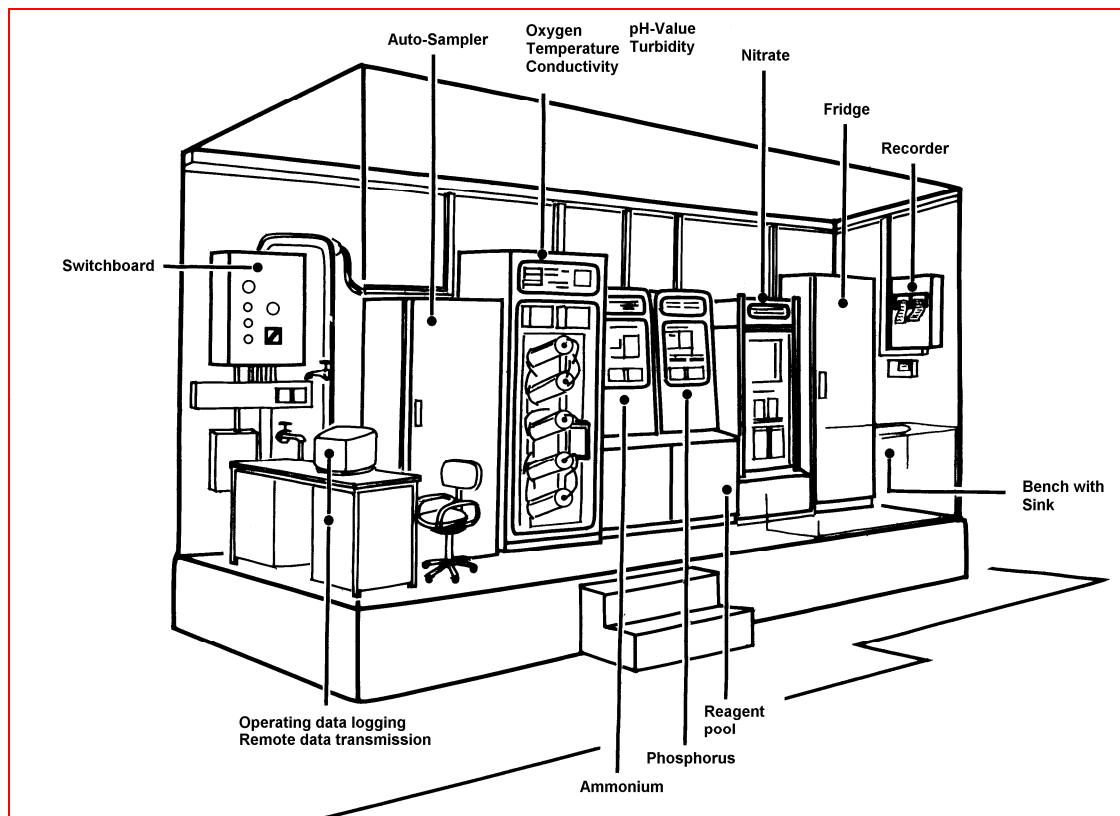
Figure 6: Water Quality Monitoring Station (On-Site Principle).
