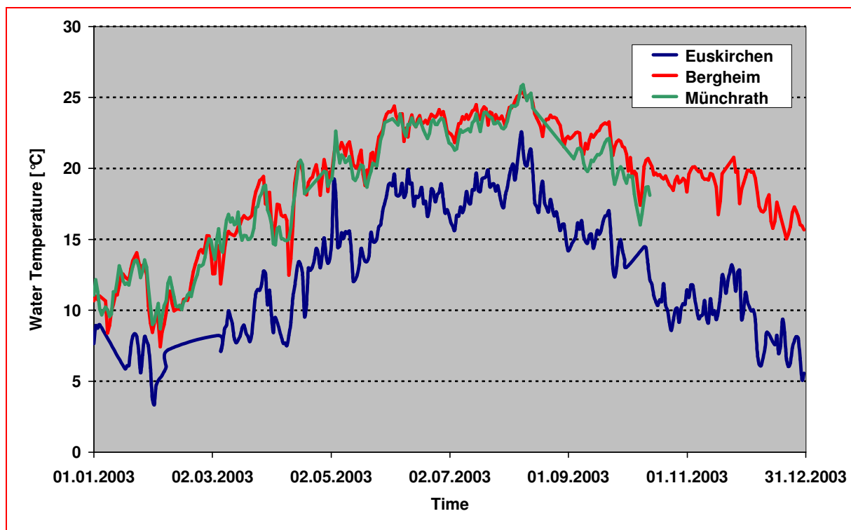
Figure 13: Water Temperature – Annual Cycle at the Upper (Euskirchen), Middle (Bergheim) and Lower Reaches (Münchrath), Year 2003.
