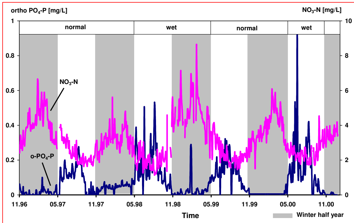
Figure 16: Nutrients - Time-Variation Curves ( o -PO 4 -P, NO 3 -N), year 1996 - 2000.
