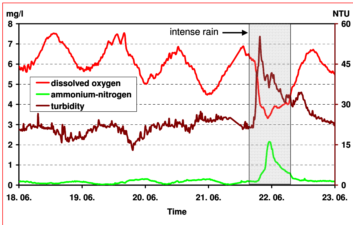
Figure 17: Results at the Bergheim Monitoring Station during Dry Weather and Sewer Overflows, Year 2000 (NTU \triangleq Nephelometric Turbidity Unit).
