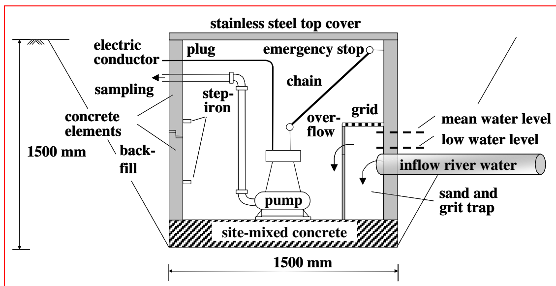
Figure 9: Pumping Station.
