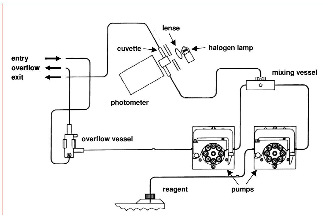
Figure 12: Photometric Measuring Instruments – Principle.
