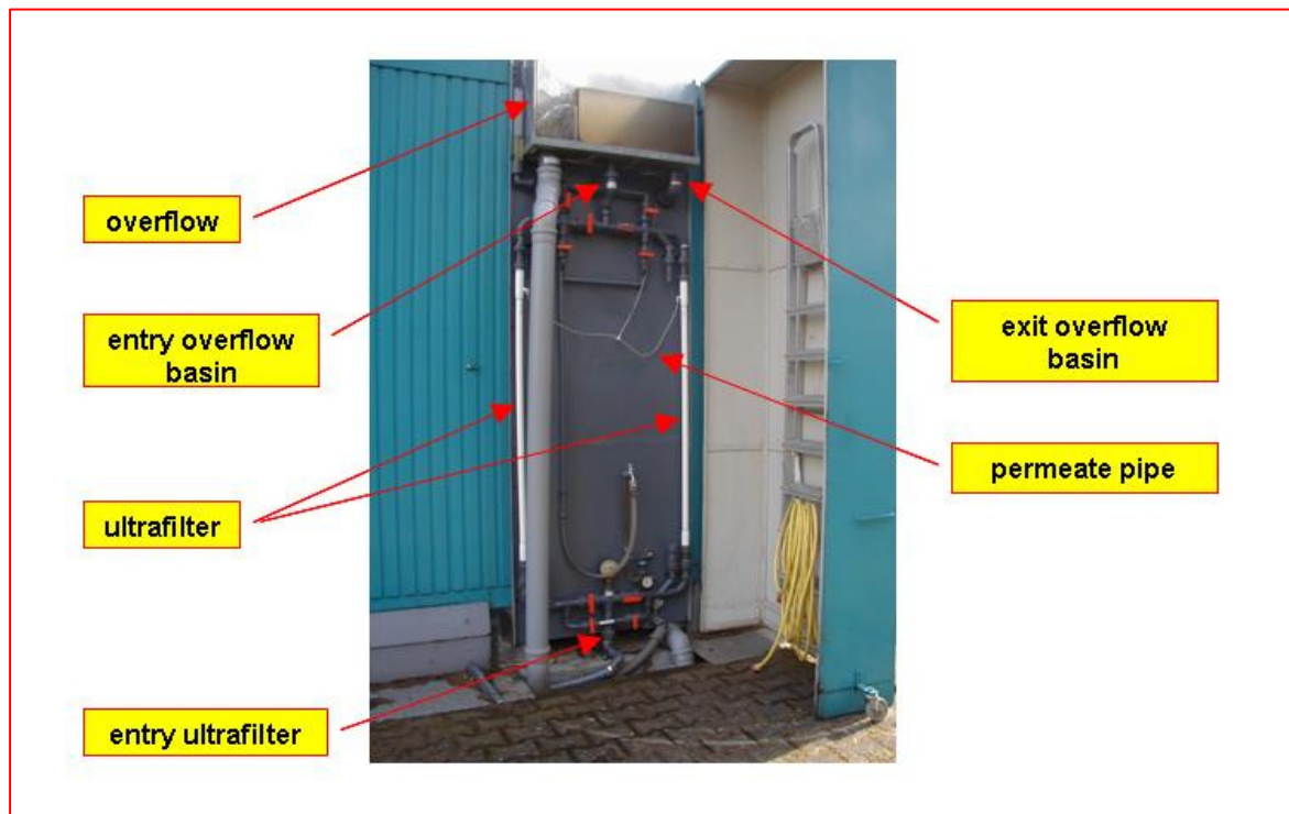
Figure 10: Pre-Treatment Unit.
