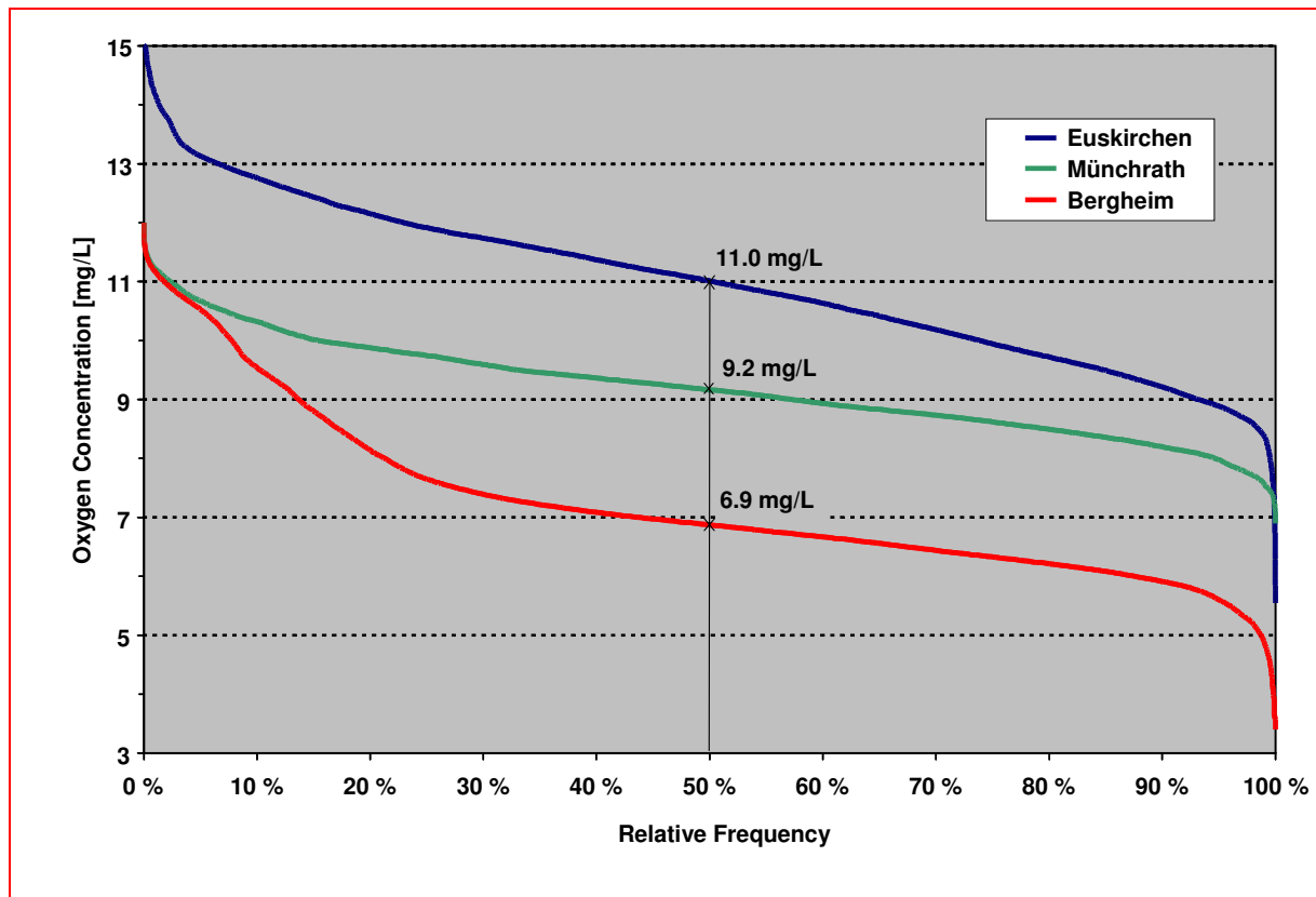
Figure 15: Oxygen Concentration - Duration Curves, Year 2003.
