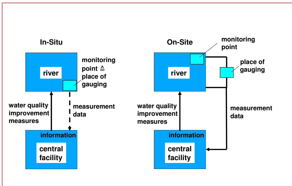
Figure 4: Online Monitoring – In-Situ and On-Site Principles.
